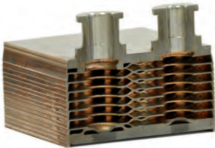
Cross-section of a brazed plate heat exchanger
